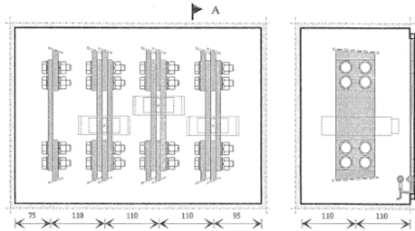
Primary busbar of CT Neutral busbar
