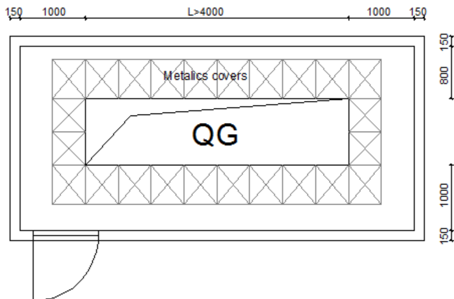
Figure 1.2 – Minimum dimensions for main low voltage switchboard installation for collective installations with back connection, with length L > 4m .
