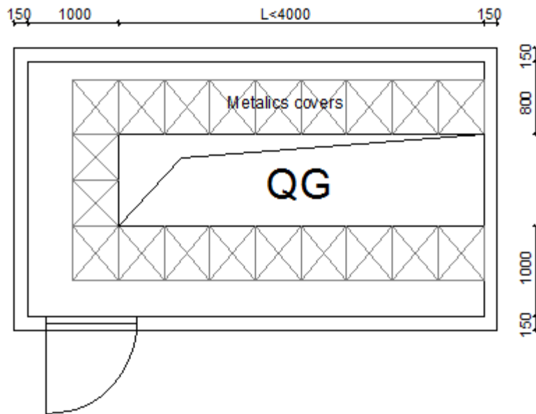
Figure 1.1 – Minimum dimensions for main low voltage switchboard installation for collective installations with back connection, with length L < 4m .
